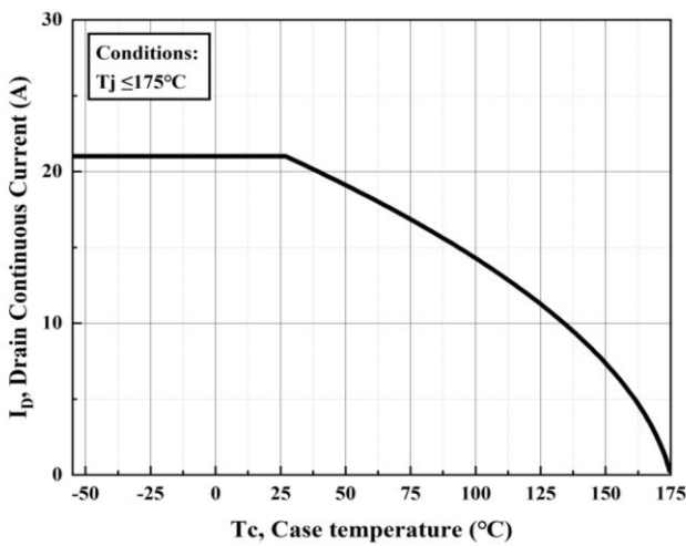
Figure 17. Continuous Drain Current Derating vs. Case Temperature
