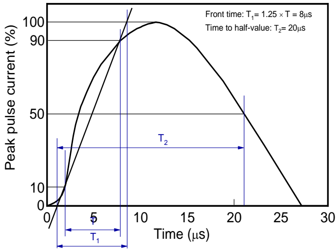
8/20 \mu s waveform per IEC61000-4-5
