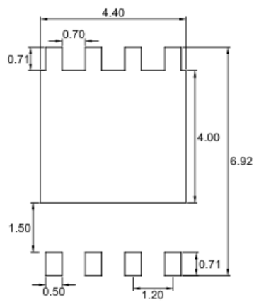
Suggested Solder Pad Layout Top View
