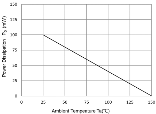
Fig 6: P_D-Ta Curve
