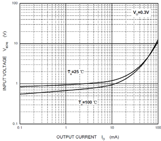
ON Characteristics
