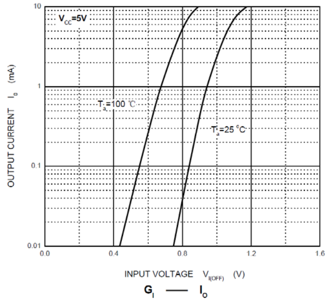
OFF Characteristics
