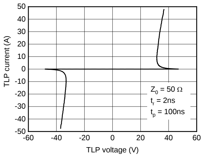
TLP Measurement
