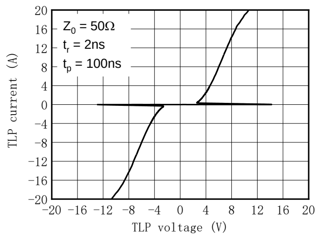
TLP Measurement
