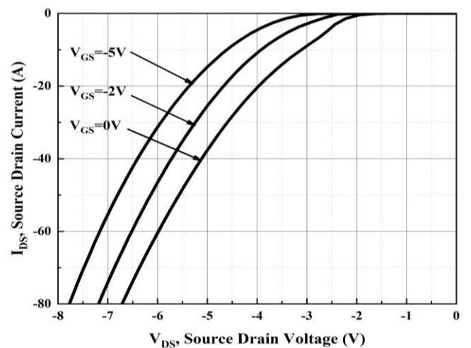
Figure 8. Body Diode Characteristic at T_j = 25^\circ\text{C}
