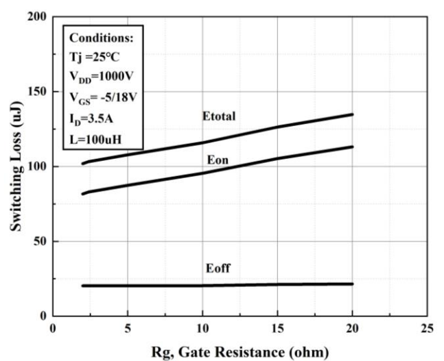
Figure 20. Clamped Inductive Switching Energy vs. R g
