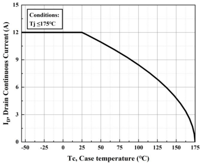
Figure 17. Continuous Drain Current Derating vs. Case Temperature
