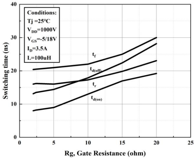
Figure 21. Switching Times vs. R_g
